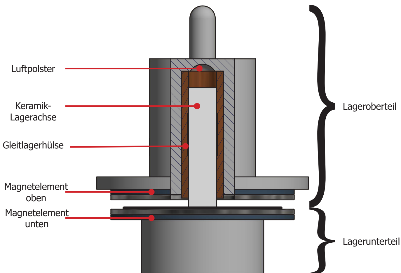
Abb. 1: clearaudio CMB-Lager
