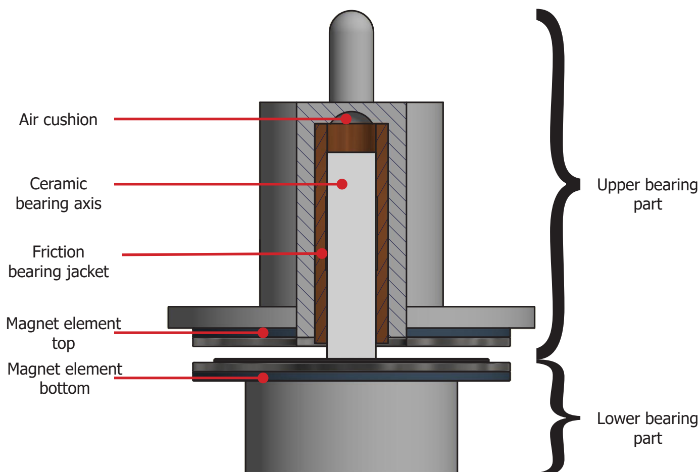
Pic. 1: Clearaudio CMB-Bearing
